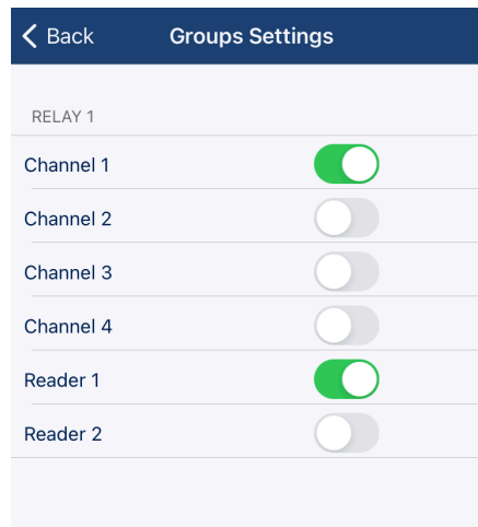
RELAY 1 setting: The illustration shows RELAY 1 will be activated when Channel 1 of a registered transmitter is activated or when a registered badge is read by Reader 1.
