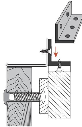
CX-DE1216 Supports en L 1-1/2" x 1-1/2"
